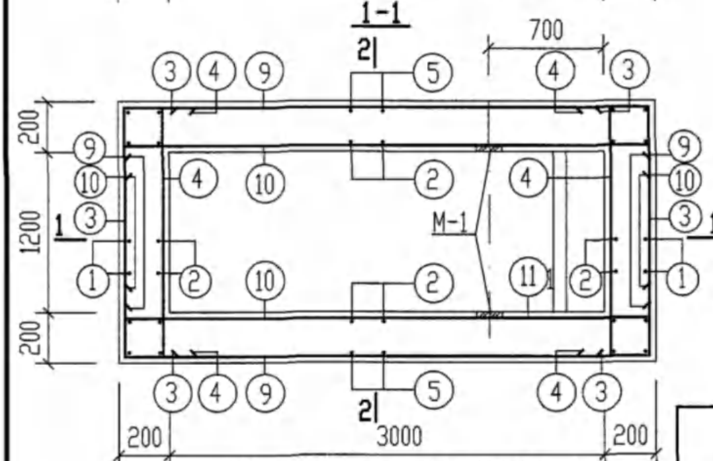
GC-1F, 1SF, 1QF, 1SQF 平面配筋图
