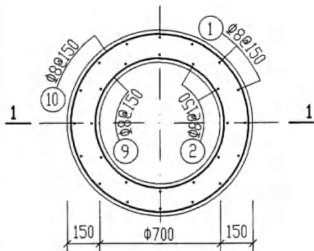
GWM-1配筋图
