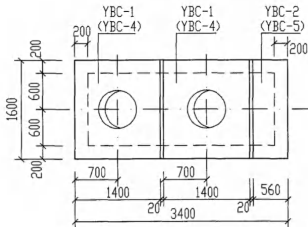
GC-1, 1S (GC-1Q, 1SQ) 盖板平面布置图
