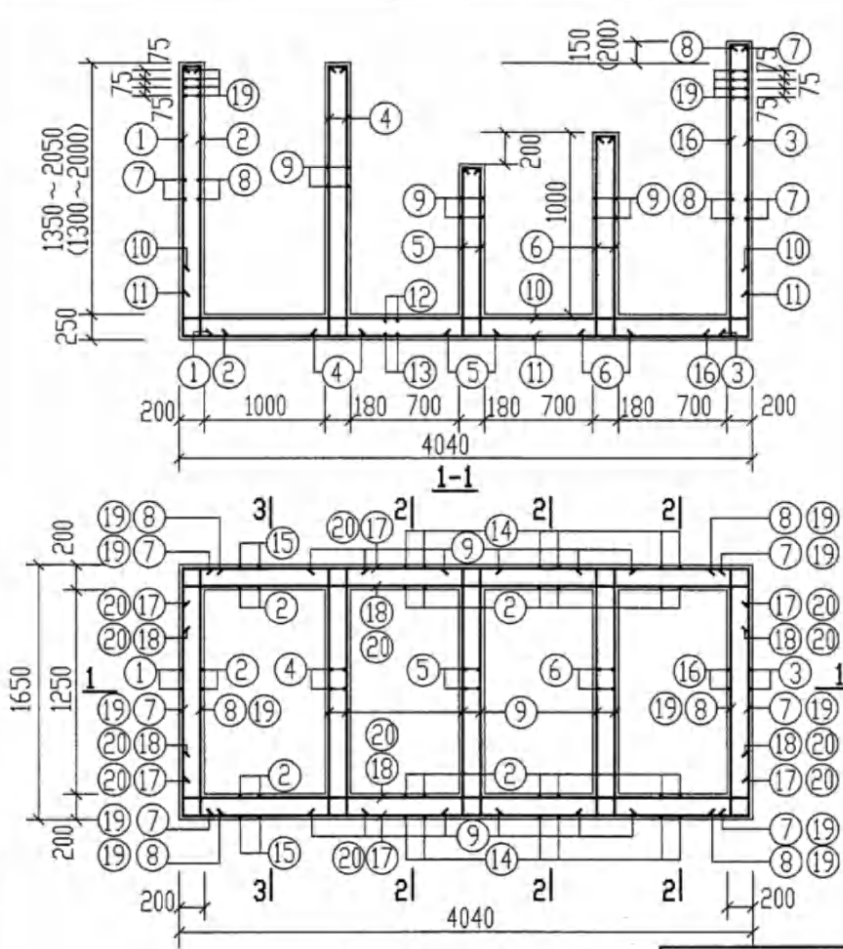
GP-1, 1S, 1Q, 1SQ 平面配筋图
