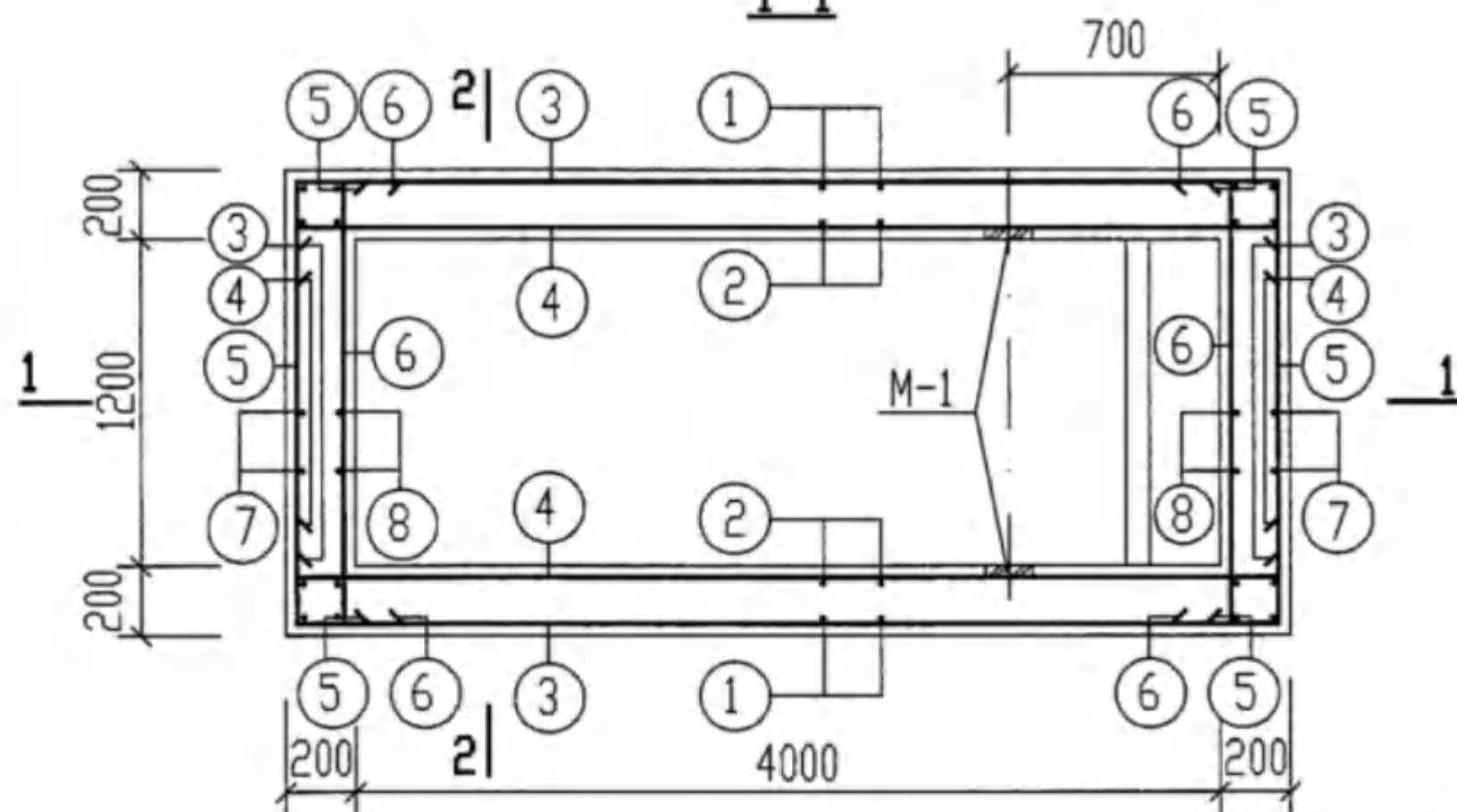
GC-2F, 2SF, (2QF, 2SQF)平面配筋图
