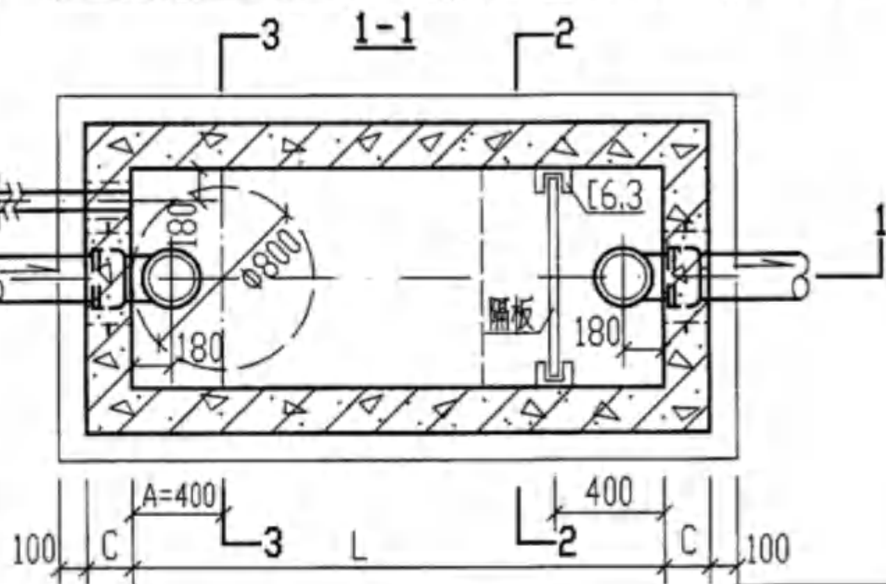
GG-2F, 2SF (GG-3F, 3SF)平面图
